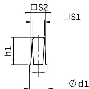
Detail B (Stem) : Mounting interface
